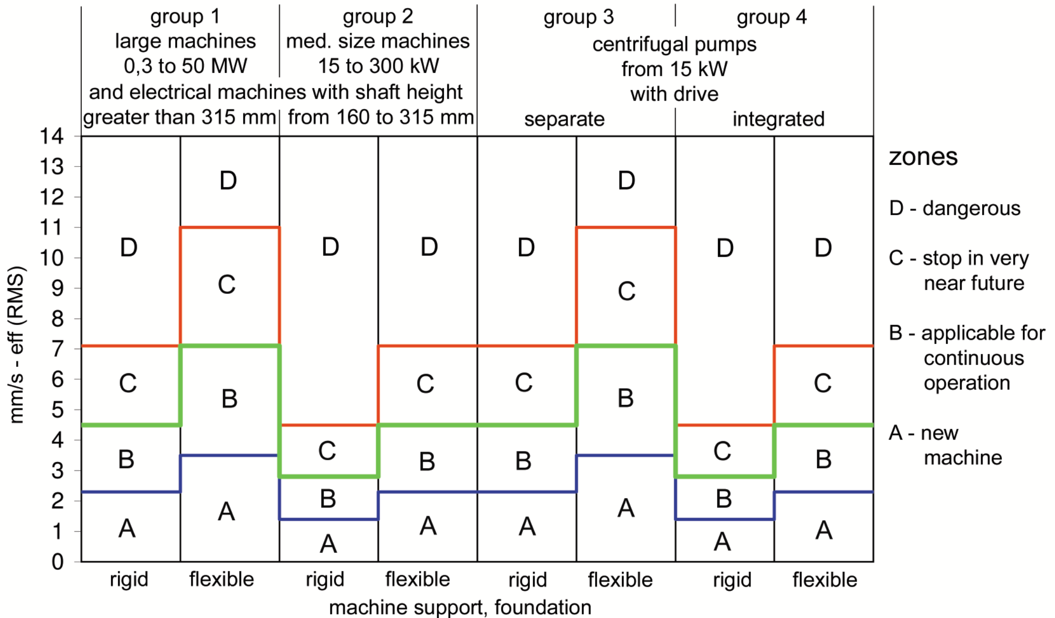
Zones for assessment of vibration severity in mm/s - eff evaluated for machines installed at site (acc. ISO 10816 - 3)
